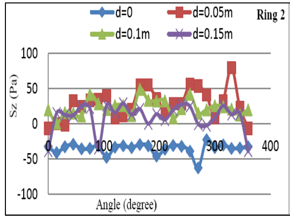
Fig 4 (A-C): Distribution of S_z , S_{yz} And S_{xz} Respectively, Along the Ring of Radius=0.4m For Various Sizes of Delamination.
