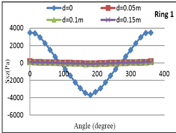
Fig 3 (A-C): Distribution of S_z , S_{yz} And S_{xz} Respectively, Along the Ring of Radius=0.3m For Various Sizes of Delamination
