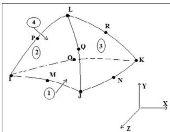
Fig1: 10 Noded Solid187 Element
